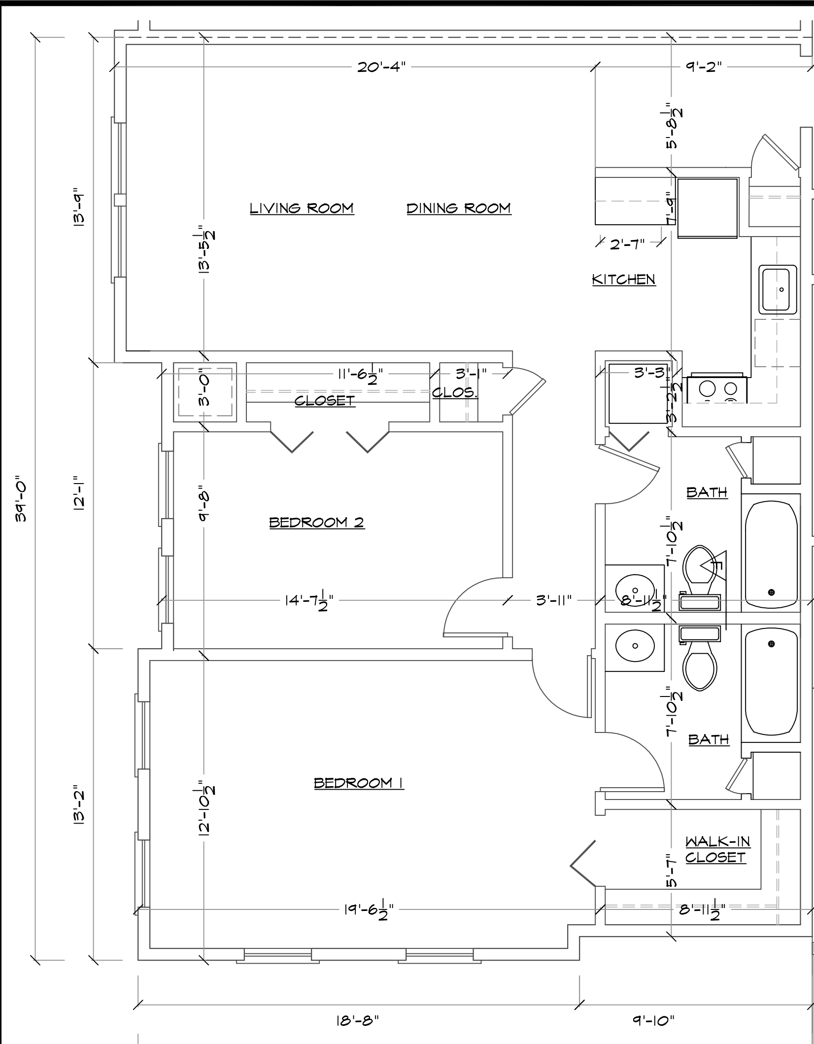
2nd & 3rd FL. TYP. 2 BED UNIT PLAN SCALE: 1/4" = 1'-0"
