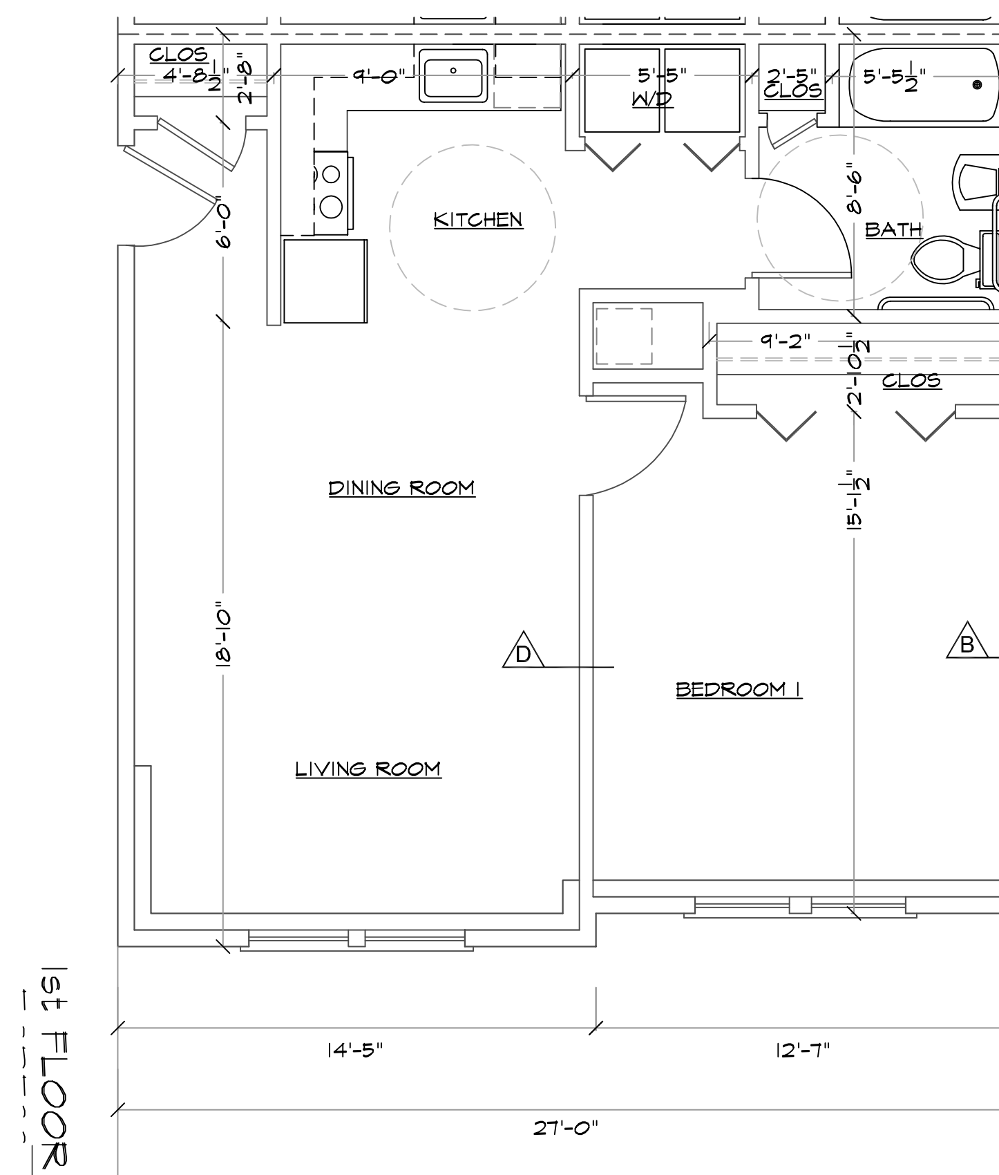
1st FL. TYP. 1 BED UNIT PLAN SCALE: 1/4" = 1'-0"
