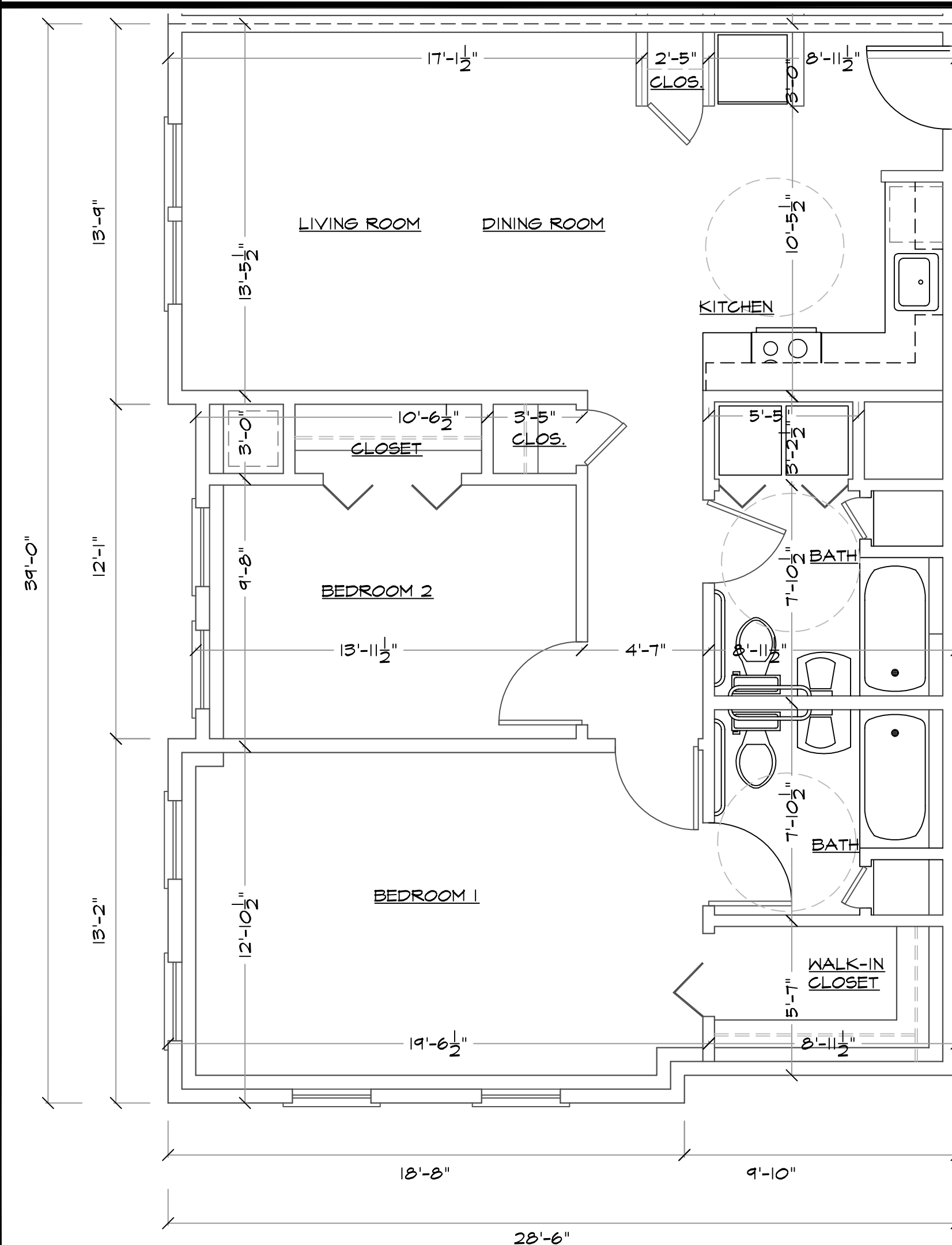
1st FL. TYP. 2 BED UNIT PLAN SCALE: 1/4" = 1'-0"
